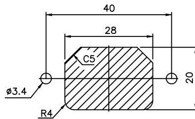
Mounting inlet flange in front of cover.
