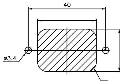
Mounting inlet flange at back of cover.
